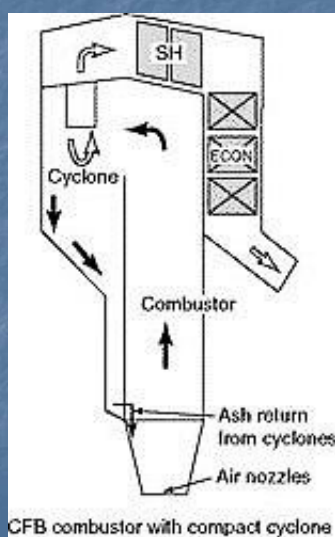
CFB combustor with compact cyclone
